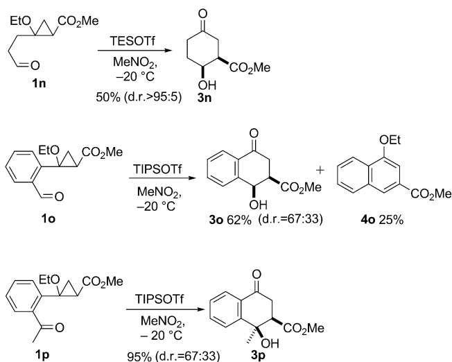
Scheme 4. Construction of skeletons with a 1,4-dioxogen-substituted cyclohexane.
